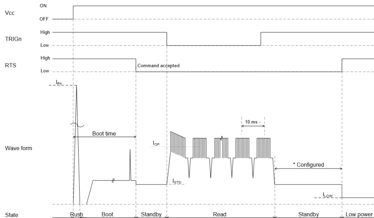
Figure 4: Current Waveform
