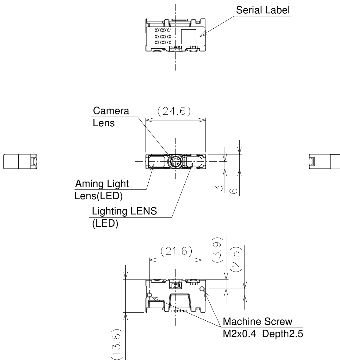
Figure 20: MDI-4000 and MDI-4050 Camera Drawing
