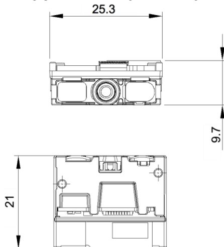
Figure 3: Dimensions of the MDI-4100 and MDI-4150
